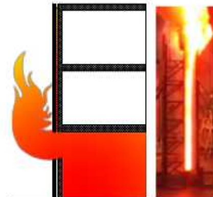
Figure 11. Fire spread through a ventilated layer in a façade [14]
