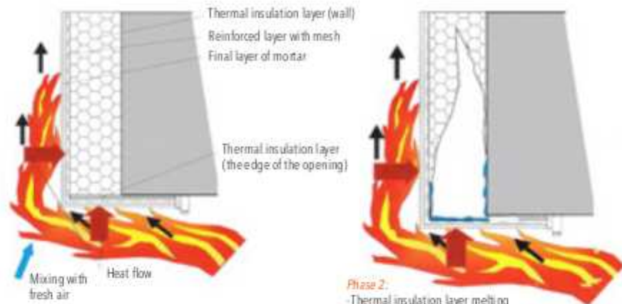
Phase 1: Thermal effect on a façade from the bottom and front side into the ETCS system.
