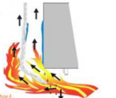
Phase 4: - Complete disintegration of the ETCS system at the edge - Separation of flaming droplets of melted material - Penetration of flame behind the plaster - Burnout of the system on the inside and external sides - Flaming droplets falling
